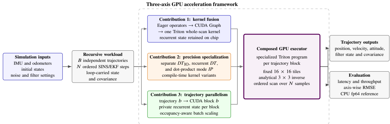
Fig. 3 Design overview of the proposed GPU acceleration framework. The recursive SINS/EKF workload is transformed along three complementary axes: whole-scan kernel fusion reduces launch and state-traffic overhead, component-aware precision specialization balances numerical stability and hardware cost, and multi-trajectory mapping exposes block-level parallelism. The three transformations are composed in one GPU executor and validated against the CPU fp64 reference.
